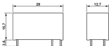
Dimensional drawing
